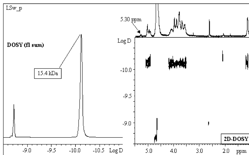
Figure 5. Projection of the diffusion dimension (left) and a 2D-DOSY experiment (right) of fraction LSw_p, performed by increasing big delta and little delta values (see Table 1). Molecular weight was derived from a calibration curve prepared with different dextrans from 10 to 500 kDa (see Table 1).
