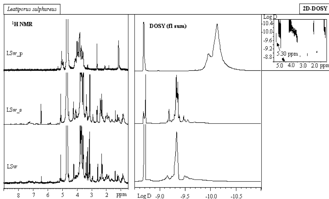
Figure 4. ^1\text{H} NMR spectra (left) and projection of the diffusion dimensions (right) on different extracts and fractions (see Table 1) of L. sulphureus . The 2D-DOSY spectrum of fraction LSw_p is also shown (right, top).
